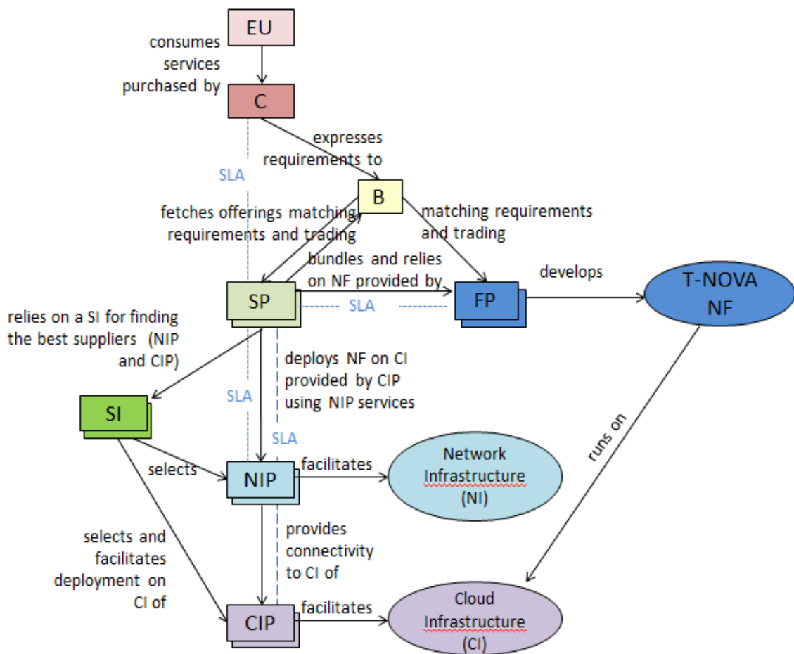
Figure 3-1 T-NOVA roles
