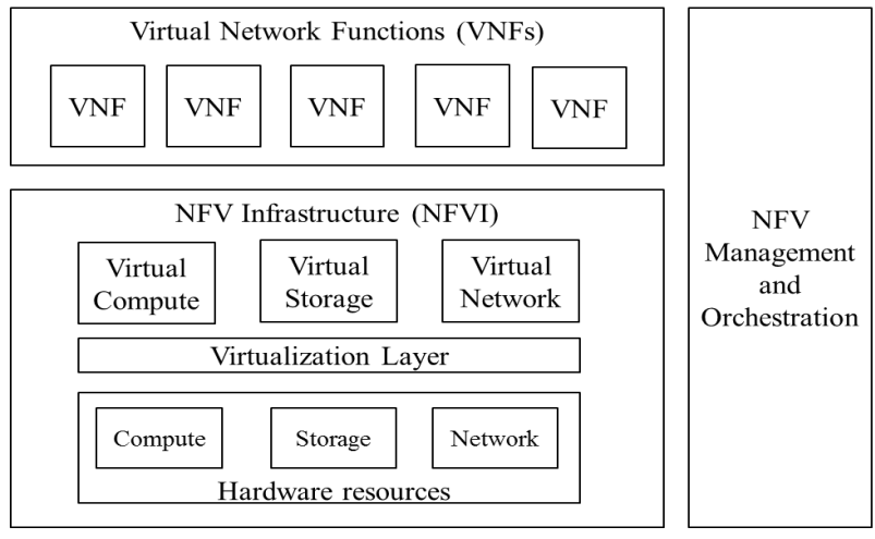
Figure 1. ETSI High-level NFV framework 1
