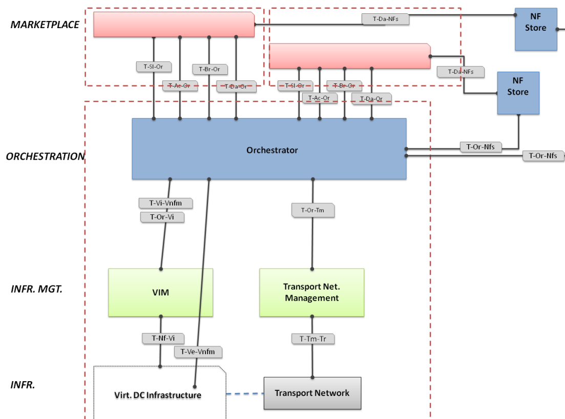
Figure 39. Architecture extension for multiple brokers under the same SP
