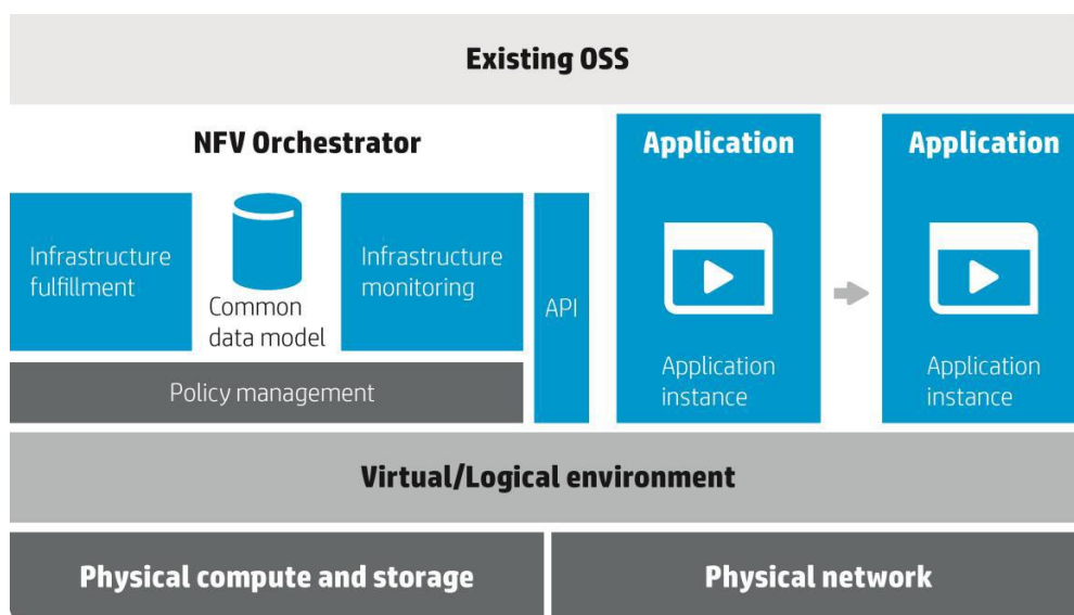
Figure 5. HP OpenNFV Functional Architecture
