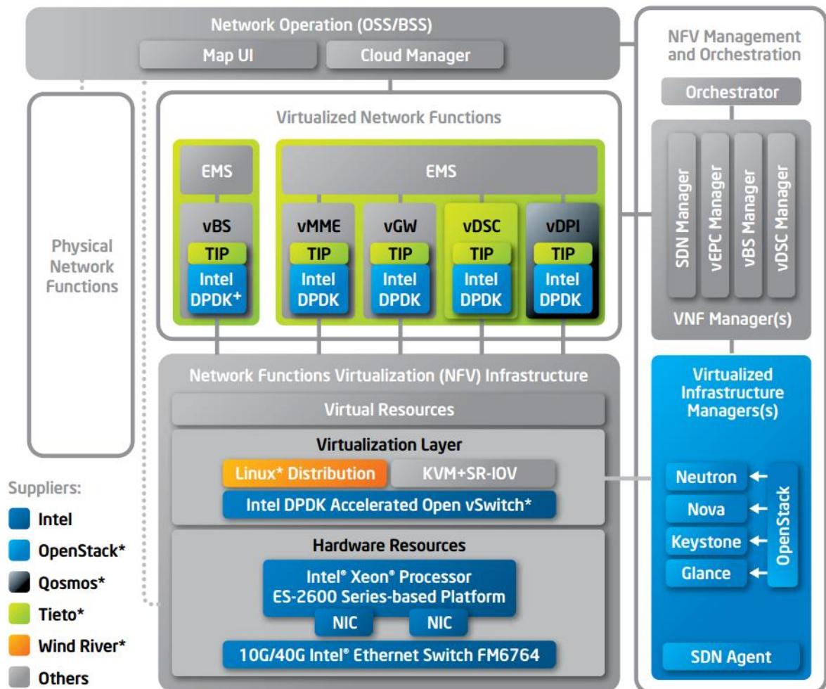
Figure 6. Intel NFV High Level Architecture
